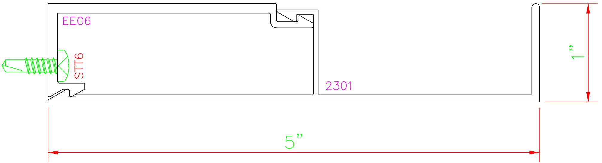
2301 / EE06 5" X 1" SNAP COVER & CLIP @ HEAD
